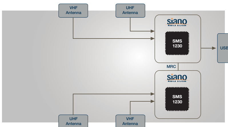
Full Diversity USB2.0HS MDTV Receiver
